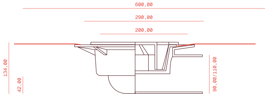
Horizontal outlet
