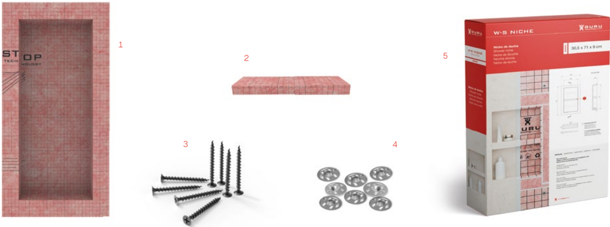
1. Prefabricated W-S Niche / 2. Divider shelf* / 3. Screws (x8) / 4. Metal washers (x8) / 5. W-S Niche Box *Not included in W-S Niche 30
