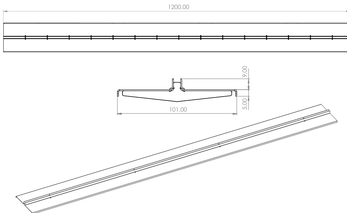
Grate Premium Unique Slot (Dimensions in mm)
