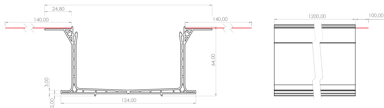
Channel (Dimensions in mm)
