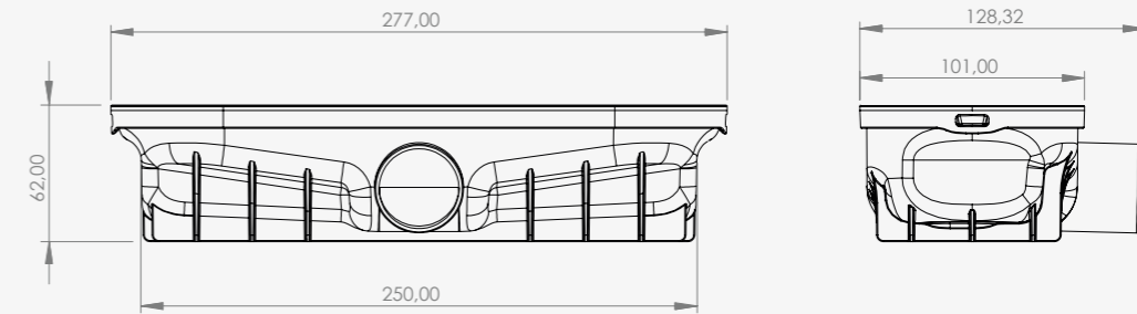
TRYPHON REDUCED: Ø 40 mm output | Connection via gluing
