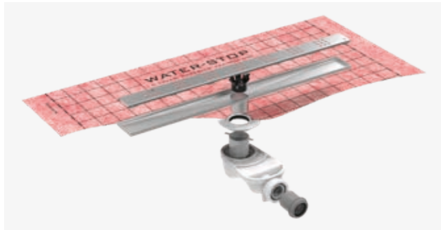
EVOLUX RUBER KIT LISA/PLUS/DARK Complete shower kit with included waterproofing.
