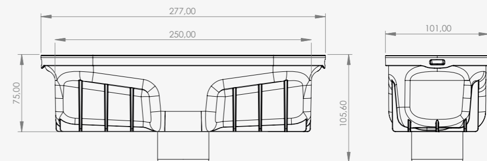
TRYPHON VERTICAL: Ø 50 mm output | Connection with pressure seal
