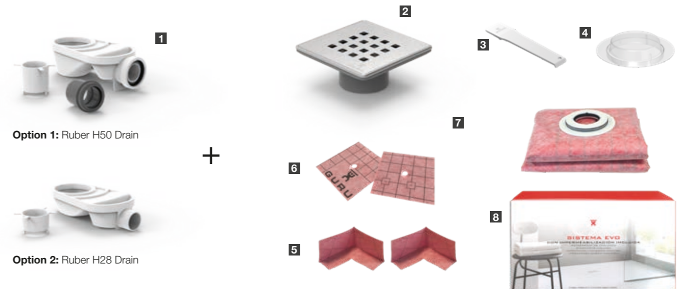
1- Drain of choice. 2- ABS cup and stainless steel grate (model of choice). 3- Grate remover. 4- Mortar level cover. 5- W-S DIN x2 (inside corners). 6- W-S TUB x2 (pass-through pipes). 7- WATER-STOP membrane with thermosealed adapter (1.5 x 2 m). 8- Evo box.
