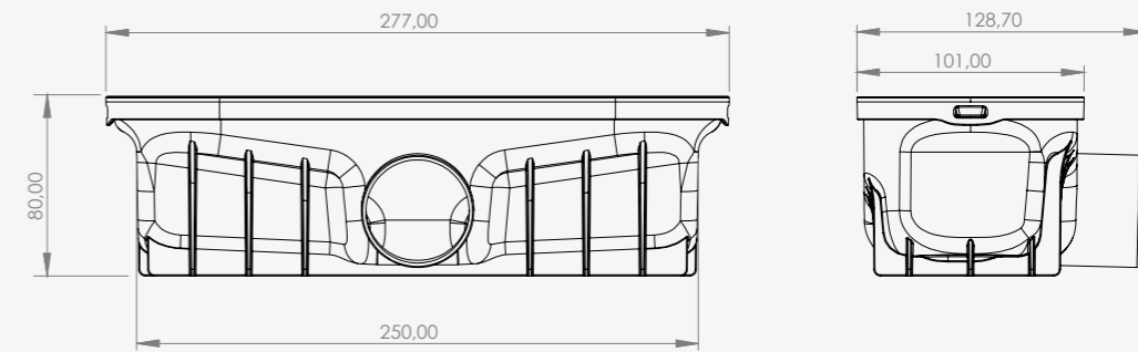
TRYPHON: Ø 50 mm output | Connection with pressure seal
